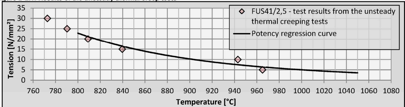
Figure D 2.1: Results of the unsteady thermal creep tests
